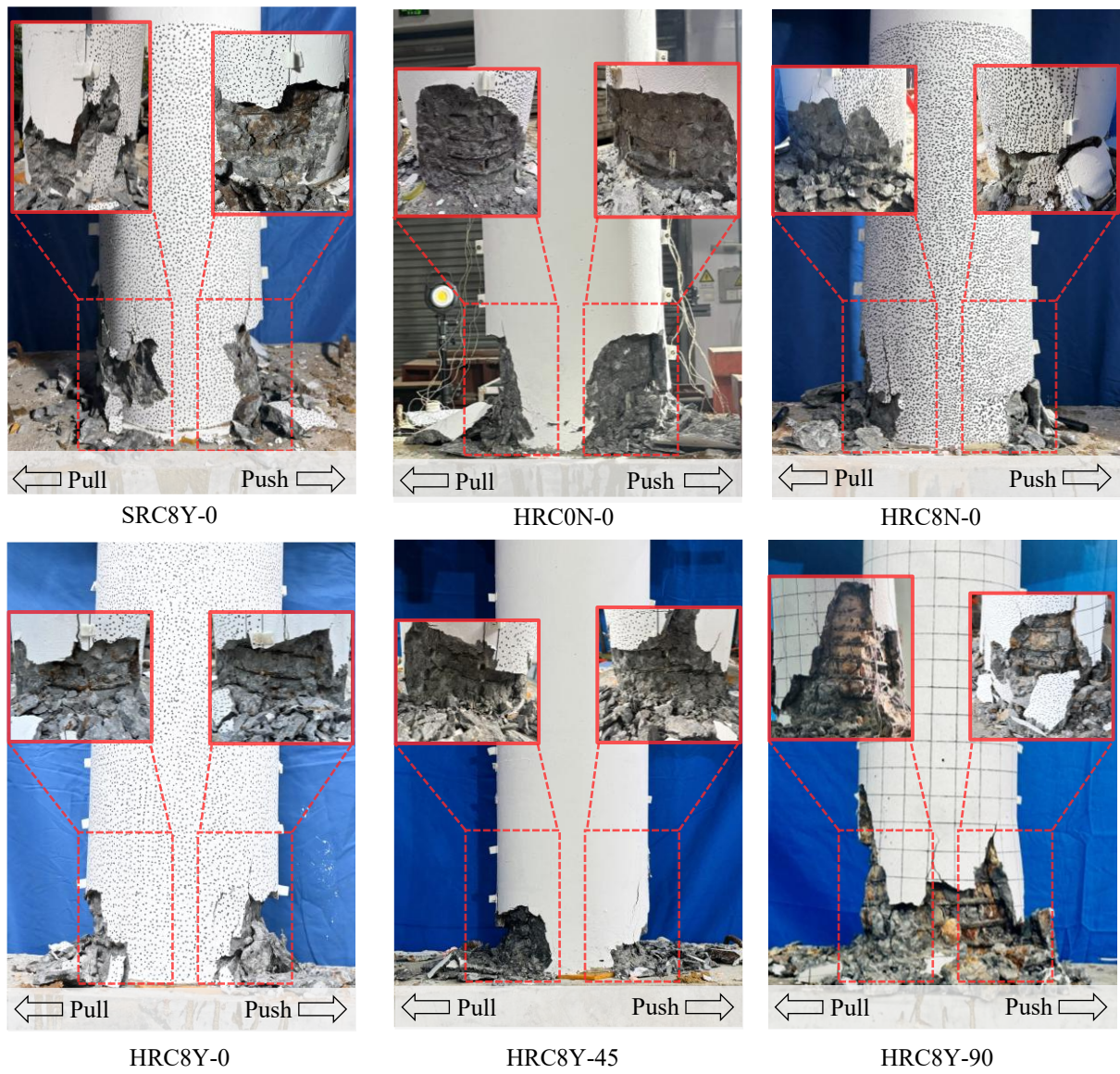
Fig. 4S. Post-test failure photographs
