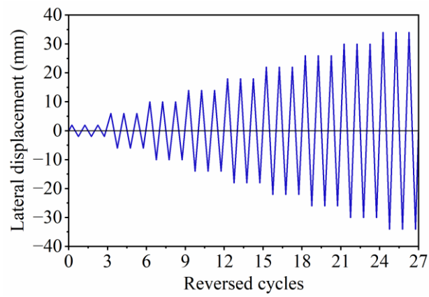
Fig. 2S. Loading protocol for reversed cyclic loading as per JGJ 2015
