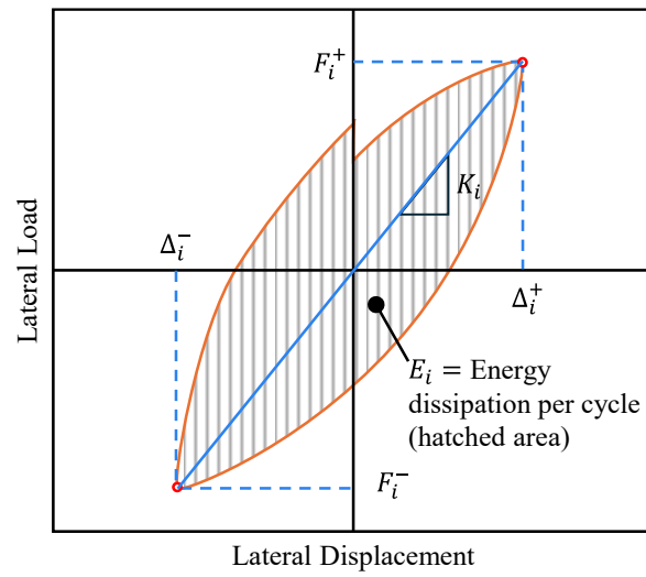
Fig. 6S. Schematic illustration of hysteresis-loop energy and stiffness calculation
