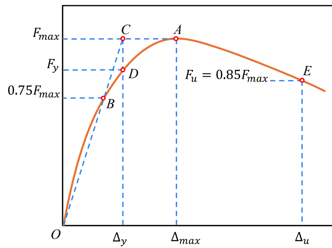
Fig. 5S. Schematic illustration of the Park method for yield point determination
