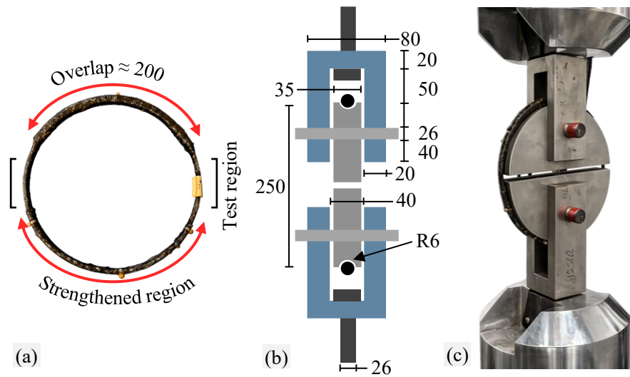
Fig. 1S. ASTM D2290 split-disk tensile test for CFRP spiral specimens: (a) CFRP spiral specimen, (b) schematic of the tensile test assembly, (c) experimental setup
